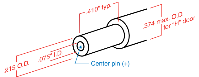
Mating Plug Dimensions and Polarity
